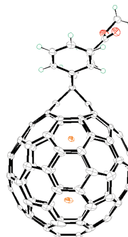
Figure 2. ORTEP view of one of the enantiomers of 2 ; the solvent molecules (i.e., \text{CS}_2 ) are omitted for clarity.
