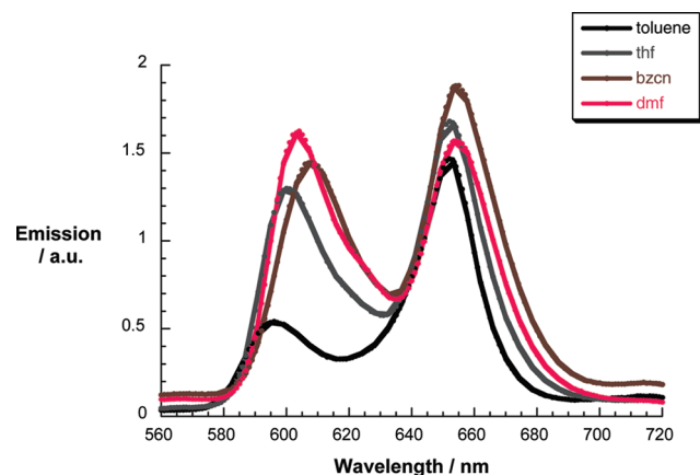
Figure 4. Steady-state fluorescence spectra of 1 in solvents of different polarity with matching absorption at the excitation wavelength (i.e., OD_{426nm} = 0.1 ).
