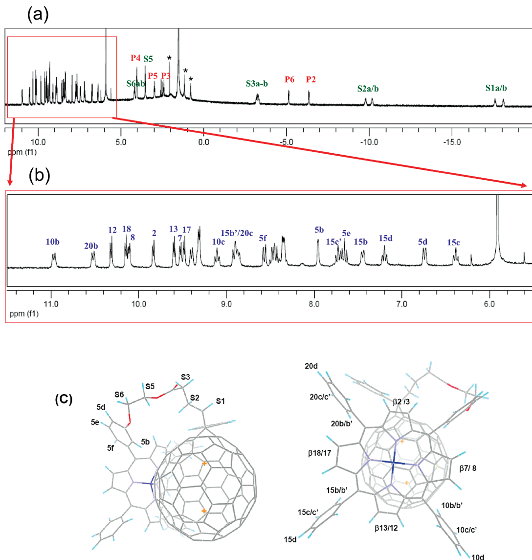
Figure 3. (a,b) ^1\text{H} NMR spectra (300 MHz) of 1 in \text{C}_2\text{D}_2\text{Cl}_4 at 293 K with the marked signals (*) originating from impurities. (c) Two side views of a molecular model of 1 . 18 The assignments are based on the 2D-DQF-COSY and NOESY experiments.
