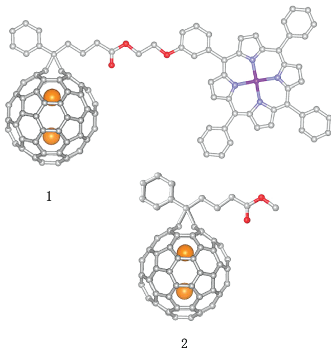
Figure 1. Structures of \text{Ce}_2@I_h\text{-C}_{80}\text{-ZnP} ( 1 ) and \text{Ce}_2@I_h\text{-PCBM} ( 2 ).
