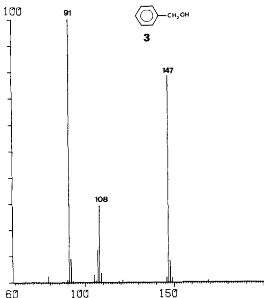
Fig. 1. CI. ( i - C_4H_{10} ) spectrum of benzyl alcohol ( 3 )
