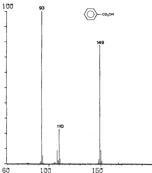
Fig. 3. CI ( i -C 4 H 10 ) spectrum of a, a -d 2 -benzyl alcohol ( 3b )
