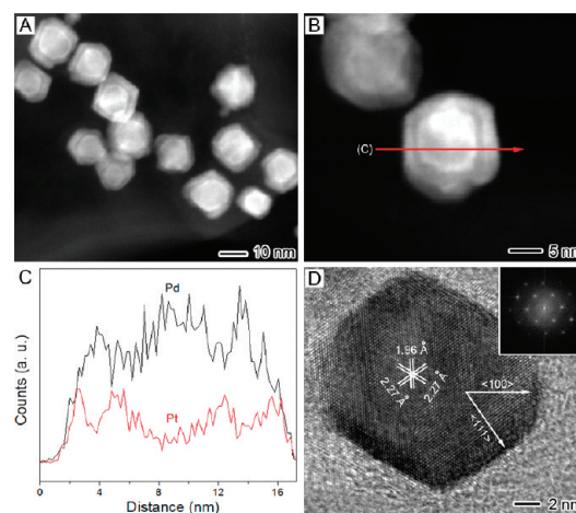
Figure 3. Morphological, structural, and compositional characterizations of the triple-shelled nanocrystals in Figure 2D, which were prepared using the standard procedure: (A, B) STEM images, (C) line-scan EDX spectrum of an individual nanocrystal as indicated in (B), and (D) high-resolution TEM image. Fourier transform (FT) pattern of an individual triple-shelled nanocrystal shown in (D) recorded along the \langle 110 \rangle zone axis.
