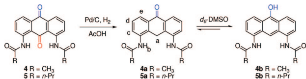
Scheme 2. Selective Catalytic Hydrogenation of Diacetamide Anthraquinones 4 and 5
