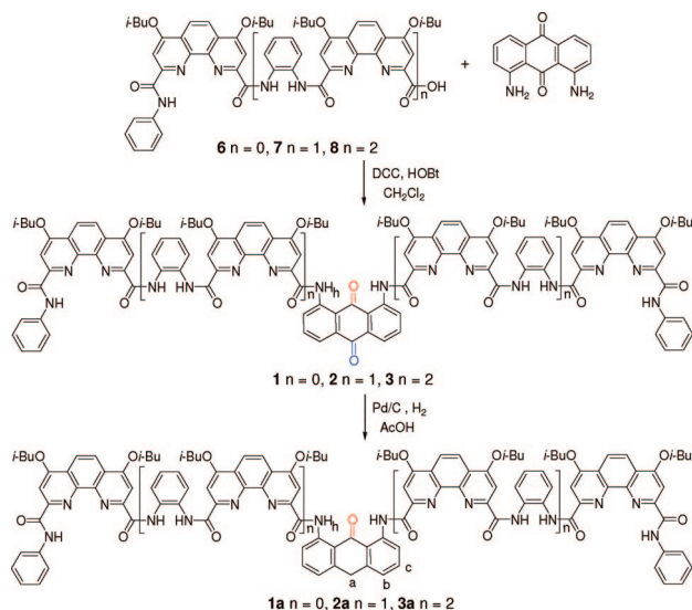
Scheme 1. Synthesis and Selective Catalytic Hydrogenations of Oligomers 1 ~ 3
