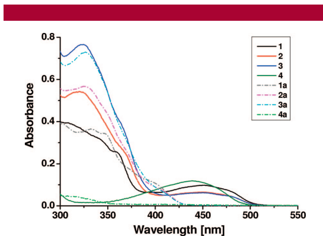
Figure 1. UV-vis spectra of the molecular strands 1 ~ 4 (solid line) and 1a ~ 4a (dash line) in CHCl 3 ( c = 1.0 × 10 −5 M).
