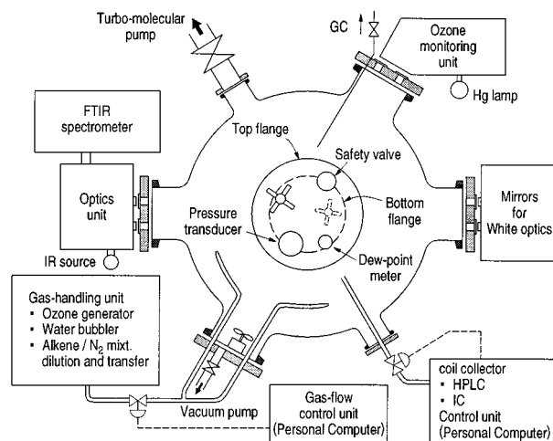
Figure 1. Schematic drawing of the 570 L glass reactor vessel.
