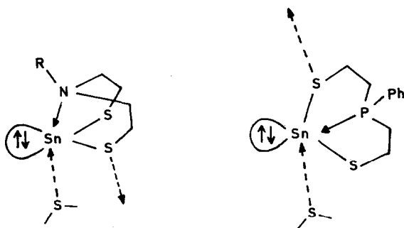
Fig. 4. Schematic representation of the \psi -trigonal bipyramidal geometry around the tin atoms in dimer a of \text{Sn}(\text{SCH}_2\text{CH}_2)_2\text{NBu}^t and in compound 1 .
