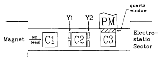
Figure 1. Schematic diagram of the experimental region of the mass spectrometer (details in text).
