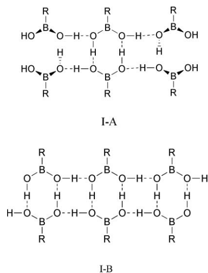
Scheme 2 Schematic representation of the interaction of homodimeric arylboronic acid dimers in the solid state. In I-A a central dimer interacts with four other dimers (only monomers are shown for clarity) which are oriented almost perpendicularly to the central dimer. In I-B each dimer is interacting with two other dimers resulting in ribbons.
