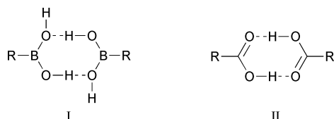
Scheme 1 Homodimeric units of boronic acids (I) and carboxylic acids (II).
