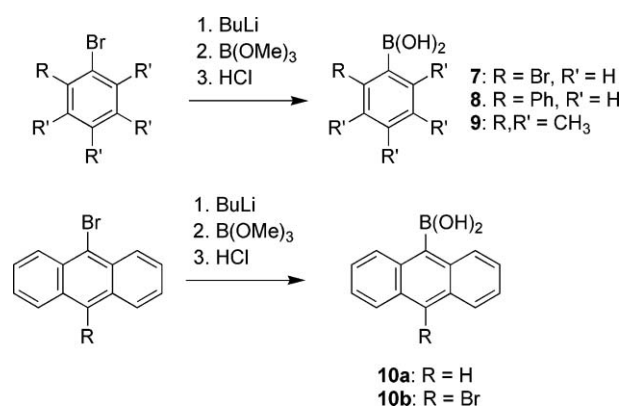
Scheme 5 General scheme for synthesis of substituted phenylboronic acids.
