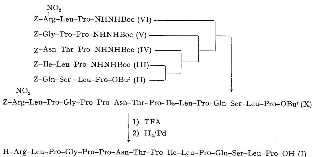
Fig. 2. Synthetic Scheme for the Peptide I
