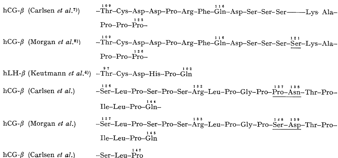
Fig. 1. Comparison of the Carboxyl-Terminal Sequences of hCG- \beta and hLH- \beta
