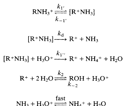
Scheme 3 Mechanism of deamination of 4,4'-dimethoxytritylammonium cations
