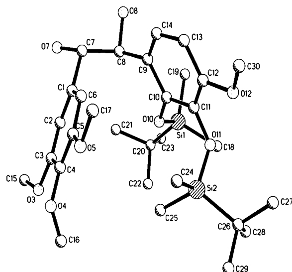
Figure 1. Crystal structure (excluding hydrogens) of ( S,S )-diol ( 8 ).
