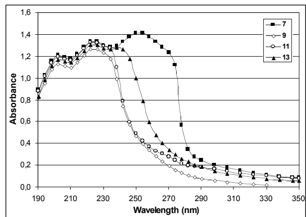
Figure 3. UV spectra of 7-phosphanorbornene derivatives (I) obtained in acetonitrile.
