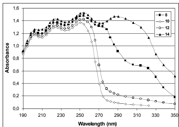
Figure 4. UV spectra of 7-Phosphanorbornene derivatives (II) obtained in acetonitrile.
