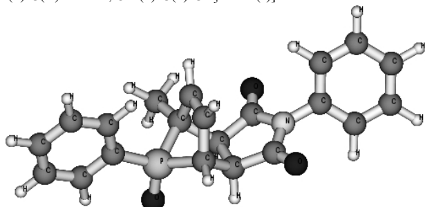
Figure 6. Perspective view of 7-phosphanorbornene 8 obtained by HF/6-31G* calculation [C(1)-C(2): 1.559, C(2)-C(3): 1.545, C(3)-C(4): 1.569, C(4)-C(5): 1.516, C(5)-C(6): 1.327, C(6)-C(1): 1.512, C(1)-P(7): 1.850, C(4)-P(7): 1.861 (Å); C(1)-P(7)-O: 116.42, C(4)-P(7)-O: 115.28, C(1)-P(7)-C(1'): 114.97, C(4)-P(7)-C(1'): 114.55, O-P(7)-C(1'): 110.51 (°)].
