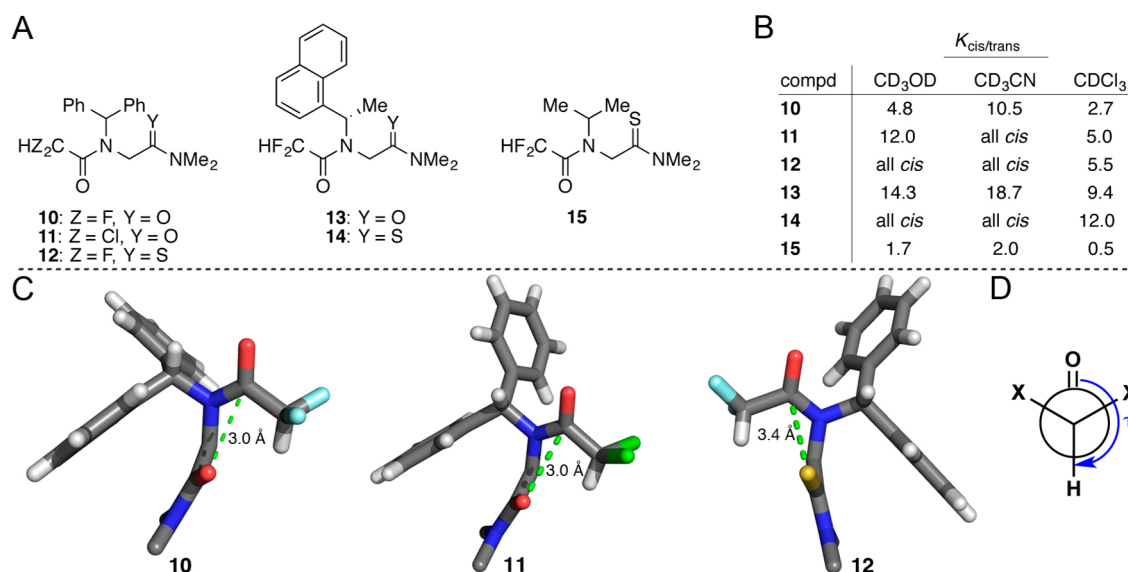
Figure 4. (A) Chemical structures of dihaloacetylated monomers. (B) K_{cis/trans} values determined by ^1H NMR. "All cis " refers to ratios above 20. (C) X-ray diffraction crystal structures of compounds 10, 11, and 12. (D) Newman projection showing the \tau angle. Atom-coloring scheme: gray, carbon; white, hydrogen; red, oxygen; blue, nitrogen; cyan, fluorine; green, chlorine; and yellow, sulfur. Hydrogen atoms in methyl and methylene groups have been removed for clarity.
