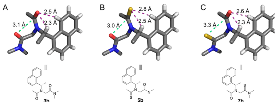
Figure 2. X-ray diffraction crystal structures of sInpe -containing compounds 3b (A), 5b (B), and 7b (C). Stick representations showing the C=O/ S_{i+1} ... C_i =O/S distance in green and distances between N-terminal carbonyls and their two closest hydrogen atoms in magenta. Atom-coloring scheme: gray, carbon; white, hydrogen; red, oxygen; blue, nitrogen; and yellow, sulfur. Hydrogen atoms in methyl and methylene groups have been removed for clarity.
