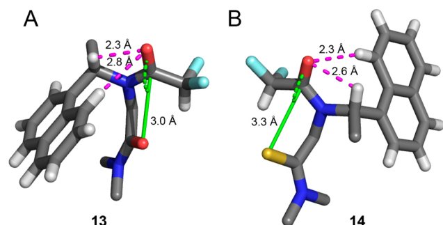
Figure 5. X-ray diffraction crystal structures of difluoroacetylated compounds 13 and 14 . Stick representations showing the C=O/ S_{i+1}\cdots C_i=O distance in green and distances between N-terminal carbonyls and their two closest hydrogen atoms in magenta. Atom-coloring scheme: gray, carbon; white, hydrogen; red, oxygen; blue, nitrogen; cyan, fluorine; green, chlorine; and yellow, sulfur. Hydrogen atoms in methyl and methylene groups have been removed for clarity.
