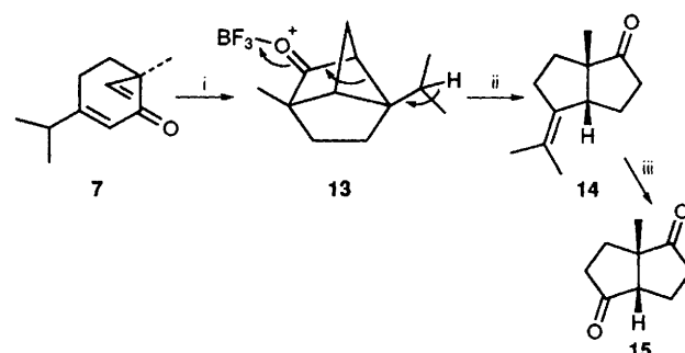
Scheme 3 Reagents and conditions: i, hν (450 W Hg lamp), pyrex, EtOAc, 87%; ii, BF 3 ·Et 2 O, CH 2 Cl 2 , room temp., 50%; iii, O 3 , CH 2 Cl 2 , -78 °C, 87% or RuCl 3 , MeCN-CCl 4 -H 2 O, NaIO 4 , 76%
