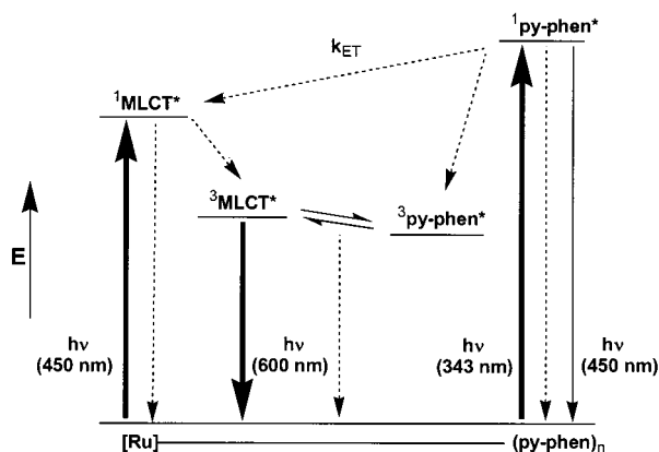
Figure 8. Energy level diagram describing the photophysical processes of [\text{Ru}(\text{bpy})_2(\text{py-phen})]^{2+} and [\text{Ru}(\text{py-phen})_3]^{2+} at room temperature. Solid lines represent radiative transitions and dashed lines represent nonradiative transitions.
