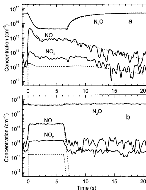
Figure 1. Time dependence of the absolute concentration of N 2 O, NO, and NO 2 , during the turn on and off of the discharge. The experimental data obtained by rapid-scan FTIR absorption spectroscopy are compared with the predictions of the present kinetic model. N 2 O starting pressure, 2 mbar; electrical power, 45 W. (a) N 2 O flow rate: 3 sccm. (b) N 2 O flow rate: 108 sccm.
