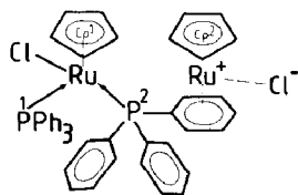
Compound VI
