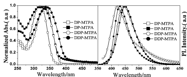
Figure 1. Absorption and fluorescence spectra of DP-MTPA and DDP-MTPA in CHCl 3 solution (hole) and solid state (solid).
