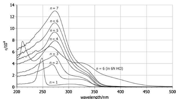
Figure 3. UV-vis spectra of 2 ( n = 1-7 ). Solvent: \text{CHCl}_3 ( n = 1-7 ) or 6 M hydrochloric acid ( n = 6 ); Concentration: 4.6-7.4 \times 10^{-6} M.
