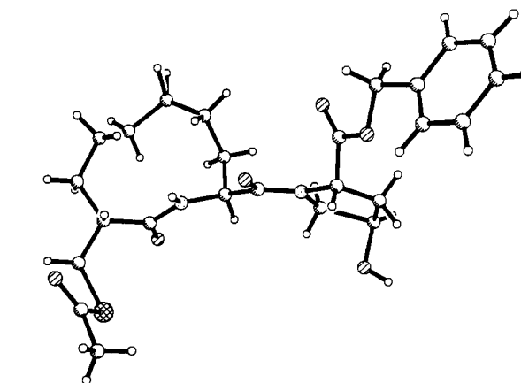
Figure 5. X-ray crystal structure of CGS 25155.
