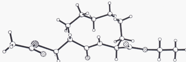
Figure 4. X-ray crystal structure of thioacetate 10.
