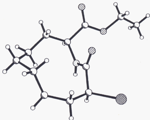
Figure 3. X-ray crystal structure of bromide 6.
