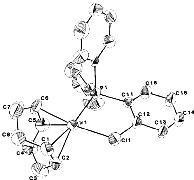
Fig. 1. The ORTEP diagram of the cation of the chelate complex [\text{Ir}(\text{cod})(\eta^2\text{-}o\text{-ClC}_6\text{H}_4\text{PPh}_2)]\text{SbF}_6 . The o\text{-BrC}_6\text{H}_4\text{PPh}_2 complex has an almost identical structure (for ORTEP diagram see ref. 4c).
