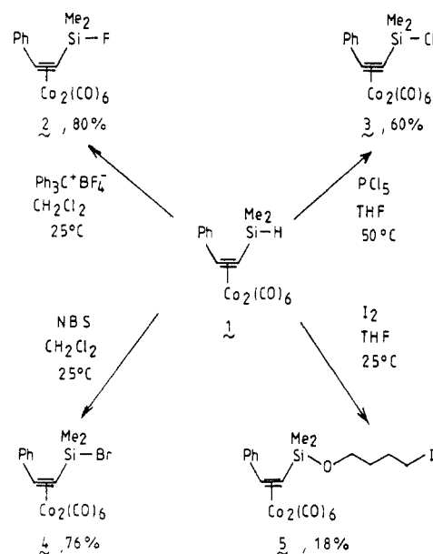
Scheme I. Halogenation Reactions of Complex 1
