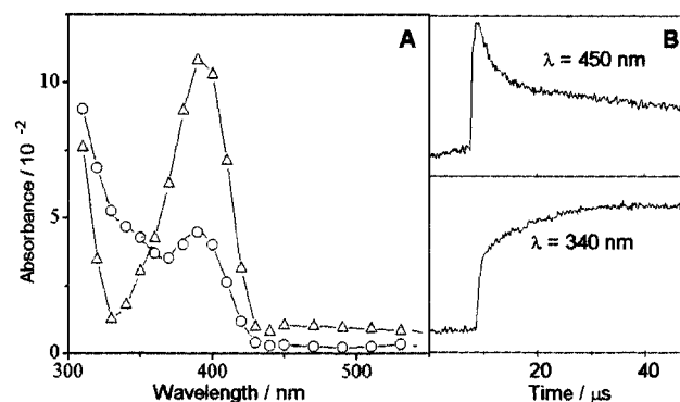
Figure 4. (A) Time-resolved absorption spectra obtained in \text{SO}_4^{\bullet-} reaction of with 4-cresol by laser flash photolysis at 2 \mu\text{s} (△) and 40 \mu\text{s} (○) after the flash. Excitation 248 nm; energy per pulse = 60 mJ; pH = 7, [solute] = 2 \times 10^{-4} \text{ M} . (B) Traces of buildup at 340 nm and decay at 450 nm measured by laser flash photolysis in 4-cresol.
