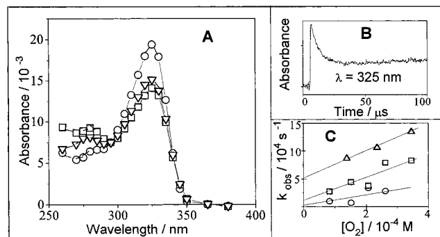
Figure 2. (A) Time-resolved absorption spectra obtained from pulse radiolysis of \text{N}_2\text{O}/\text{O}_2 (4:1 v/v) saturated solutions of 3-chlorotoluene at 3 (○), 40 (▽), and 90 \mu\text{s} (□). Dose per pulse = 600–700 rad. (B) Decay trace at 325 nm in the presence of \text{O}_2 in 3-cresol. (C) Plot of k_{\text{obs}} as a function of [\text{O}_2] in (○) 2- and (△) 3-chlorotoluenes and (□) 3-cresol.
