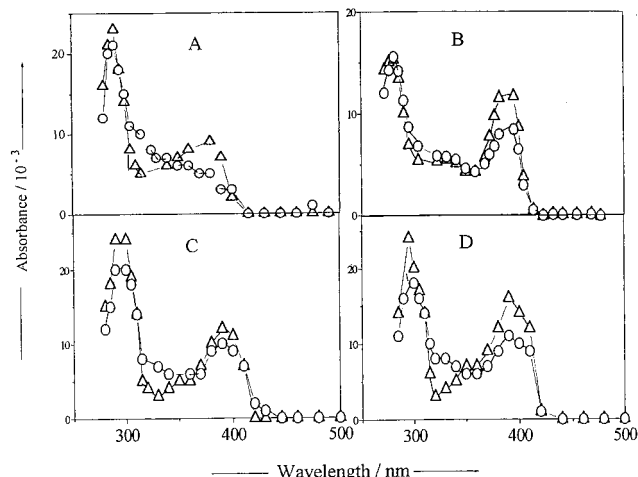
Figure 3. (A) Time-resolved transient absorption spectra obtained in \text{SO}_4^{\bullet-} reaction with (A) 2-, (B) 3-, and (C) 4-cresols at pH = 7. (D) 4-cresol at pH = 9 at 2 \mu\text{s} (△) and 40 \mu\text{s} (○) after the pulse. Dose per pulse = 1.4 krad, [solute] = 10^{-3} \text{ M} .
