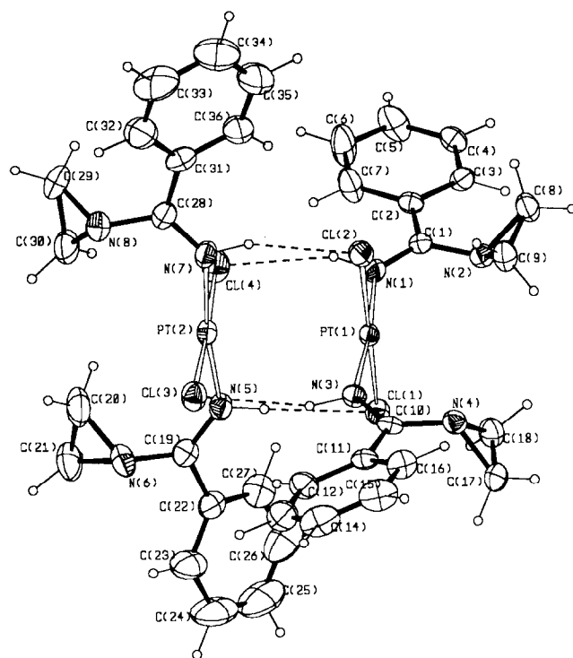
Fig. 1. An ORTEP drawing of the complex \text{trans-[PtCl}_2\text{N(H)C(Ph)NCH}_2\text{CH}_2\text{]}_2 ( 3 ) with the atom-numbering scheme.
