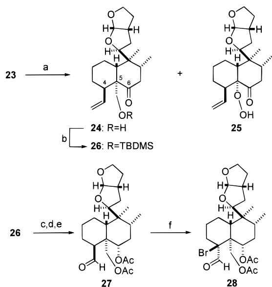
Scheme 7 a
