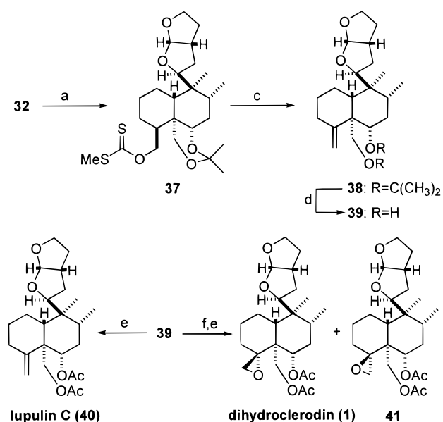
Scheme 9 a
