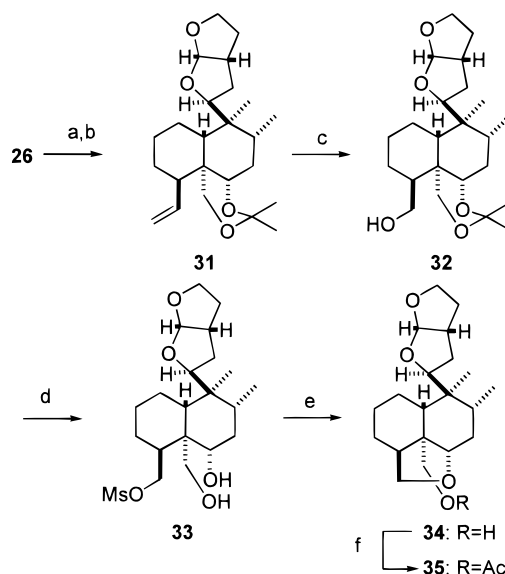
Scheme 8 a
