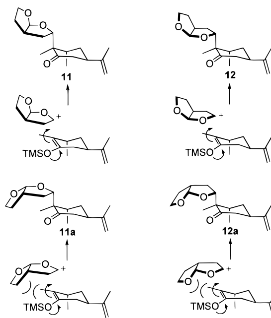
Scheme 3
