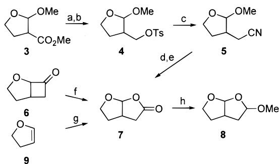
Scheme 2 a
