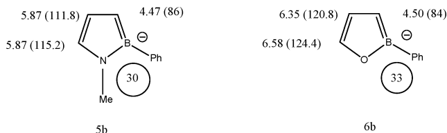
Figure 1. Comparison of the 1 H NMR, 13 C NMR (in parentheses), and 11 B NMR (in circles) chemical shift values of 5b and 6b in THF- d 6 .
