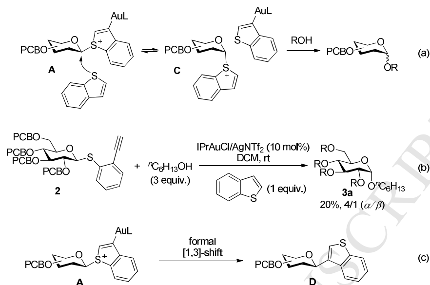
Scheme 3. Involvement of benzothiophene byproduct in the reaction
