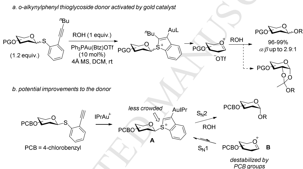
Scheme 2. Redesigning o -Alkynylphenyl thioglycoside donors.
