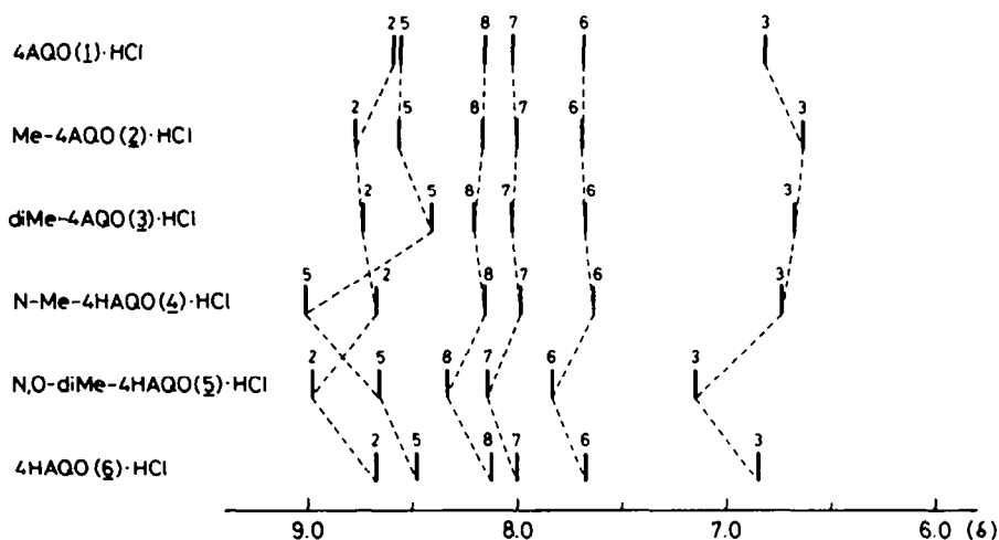
Fig. 2. Schematic presentation of chemical shift ( \delta value) of the aromatic protons of hydrochlorides of 4-substituted quinoline 1-oxides measured in (\text{CD}_3)_2\text{SO} .
