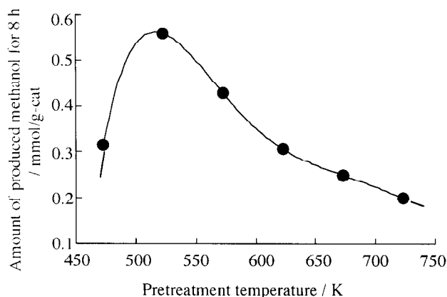
Figure 2. Dependence of the activity of methanol production from the hydrogenation of CO over the Cu- \text{Yb}_2\text{O}_3 catalyst upon pretreatment temperature. The reaction was carried out at 473 K.
