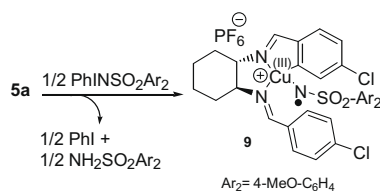
Scheme 6. Possible C–H activation product.
