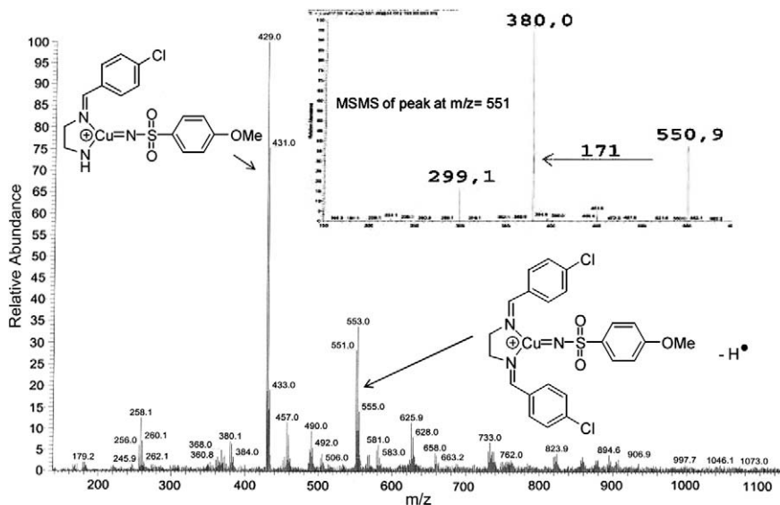
Figure 2. Positive-ion electrospray mass spectrum of the cationic portion of complex 5d-H and in the inset MS/MS spectrum of the peak at m/z = 551.
