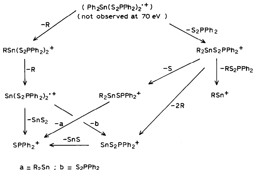
Fig. 2. Fragmentation pattern of R_2Sn(S_2PPh_2)_2 .
