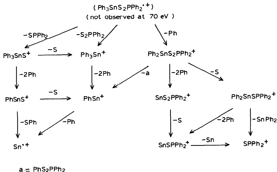
Fig. 1. Fragmentation pattern of \text{Ph}_3\text{SnS}_2\text{PPh}_2 .
