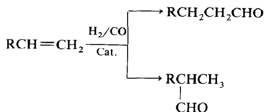
Fig. 1. Cat. = trans -[PtCl(COC 2 H 5 )(PPh 3 ) 2 ] ( 1 ); trans -PtCl(COC 2 H 5 )(PMePh 2 ) 2 ] ( 2 ); trans -[PtCl(COC 2 H 5 )(PMe 2 Ph) 2 ] ( 3 ); cis -[PtCl 2 (PPh 3 ) 2 ] ( 4 ); trans -[PtHCl(PPh 3 ) 2 ] ( 5 ); trans -[PtHCl(PEt 3 ) 2 ] ( 6 ).
