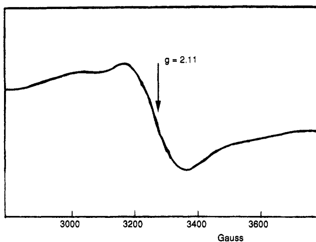
Figure 10. The ESR spectrum of catalyst after addition of \text{NaIO}_4 and water. The sample was prepared by addition of an excess of \text{NaIO}_4 and water to QSiRuW dissolved in 1,2-dichloroethane at 60 °C, and the spectrum was taken at 100 K.
