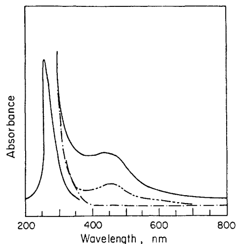
Figure 9. The UV-vis spectra of QSiRuW in the presence of (\text{C}_4\text{H}_9)_4\text{IO}_4 : (—) QSiRuW; (---) QSiRuW + (\text{C}_4\text{H}_9)_4\text{NIO}_4 ; (-.-) QSiRuW + (\text{C}_4\text{H}_9)_4\text{NIO}_4 and \text{H}_2\text{O} .
