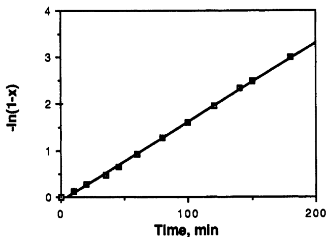
Figure 4. The reaction profile for the oxidation of styrene (first order). Reaction condition: 1 mmol of styrene, 0.001 mmol of QSiRuW, 5 mmol of \text{NaIO}_4 , 5 mL of 1,2-dichloroethane, and 5 mL of water, temperature 60 °C.
