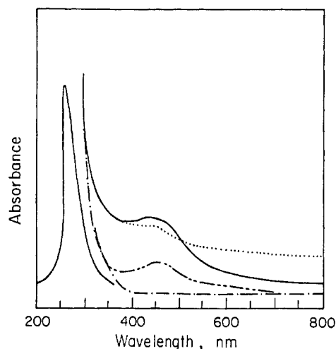
Figure 2. UV-vis spectra of the QSiRuW catalyst: (—) QSiRuW; (---) QSiRuW + KHSO 5 ; (...) QSiRuW + t -BuOOH; - · - QSiRuW + PhIO or NaIO 4 .
