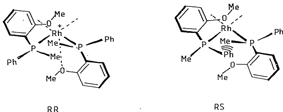
Fig. 1. Steric interactions in cis -chelated square-planar complexes of RR -4 and RS -4.
