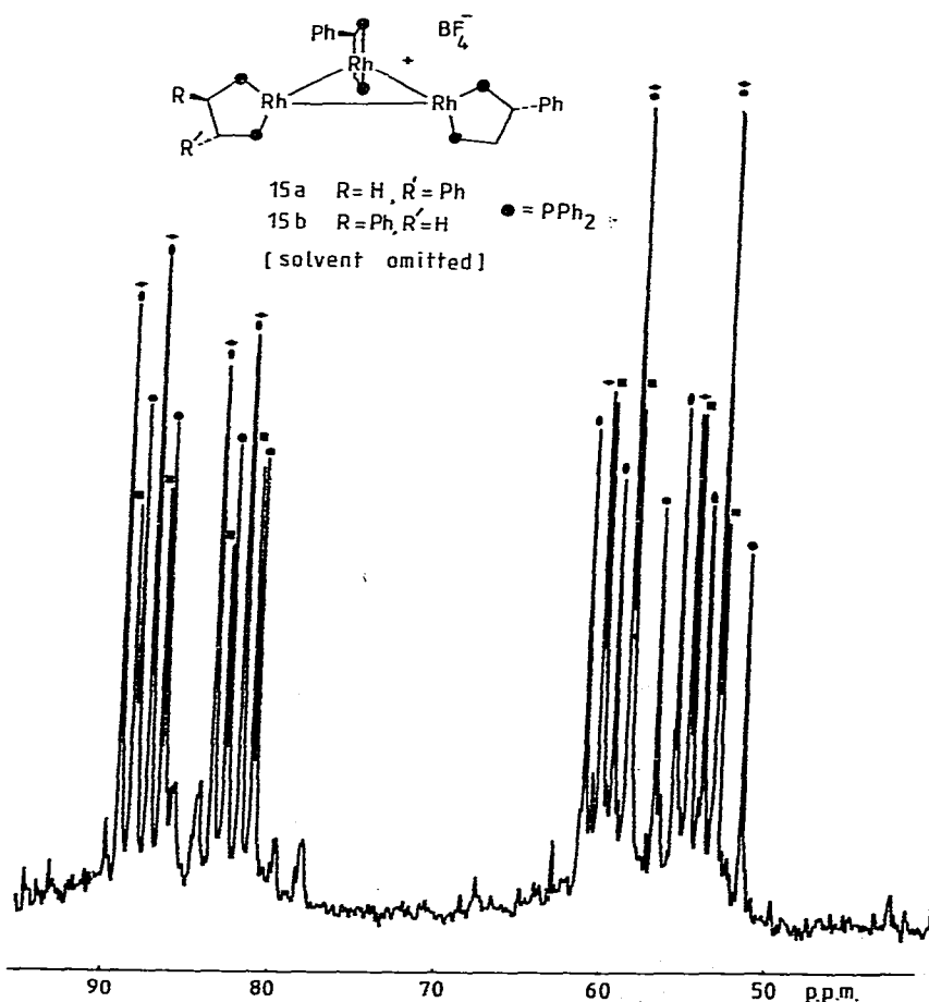
Fig. 3. ^{31}\text{P} NMR spectrum of trimers 15a and 15b in \text{CH}_3\text{OH} ; \bullet , \circ , \blacksquare , \square , are 8-line multiplets.
