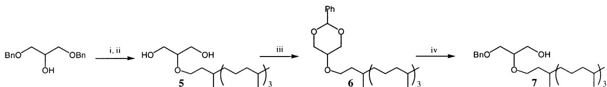
Scheme 2. (i) Phytanyl bromide, KOH, PhCH 3 ; (ii) H 2 , Pd/C, MeOH; (iii) PhCHO, p -TSA, PhCH 3 ; (iv) DIBALH, PhCH 3 /CH 2 Cl 2
