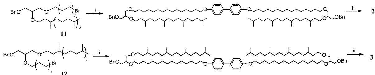
Scheme 5. (i) 4,4'-biphenol, NaH, DMF; (ii) H 2 , Pd/C, MeOH/CH 2 Cl 2
