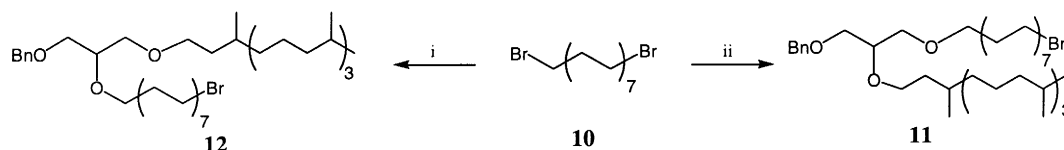
Scheme 4. (i) 9 , KOH, PhCH 3 ; (ii) 7 , NaH, THF
