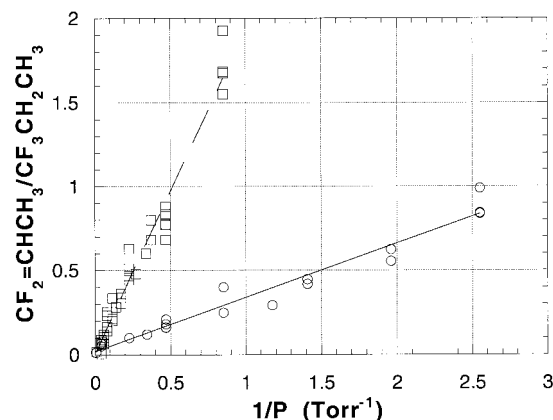
Figure 1. A plot of [\text{CF}_2=\text{CHCH}_3]/[\text{CF}_3\text{CH}_2\text{CH}_3] versus reciprocal pressure for the four-centered elimination of HF from chemically activated \text{CF}_3\text{CH}_2\text{CH}_3 with 95 kcal/mol (circles) and 101 kcal/mol (squares) of internal energy. The slope is 1.94 Torr, the intercept is 0.004 37, and the correlation coefficient is 0.983 at the higher energy, and the values are 0.321 Torr, 0.0188, and 0.979, respectively, for \text{CF}_3\text{CH}_2\text{CH}_3 with 95 kcal/mol of energy.
