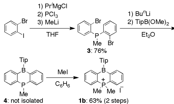
Scheme 2. Synthesis of phosphonioborin 1b .
