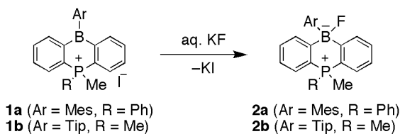
Scheme 1. Complexation of phosphonioborin 1 with fluoride ion under biphasic condition.
