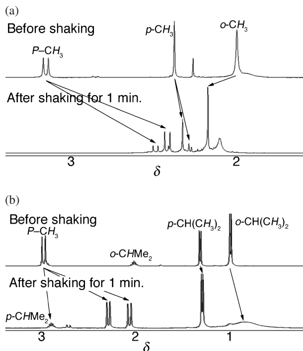
Figure 2. 1 H NMR spectral change upon mixing CDCl 3 solution of the phosphonioborins with D 2 O solution of KF. (a) 1a . (b) 1b .
