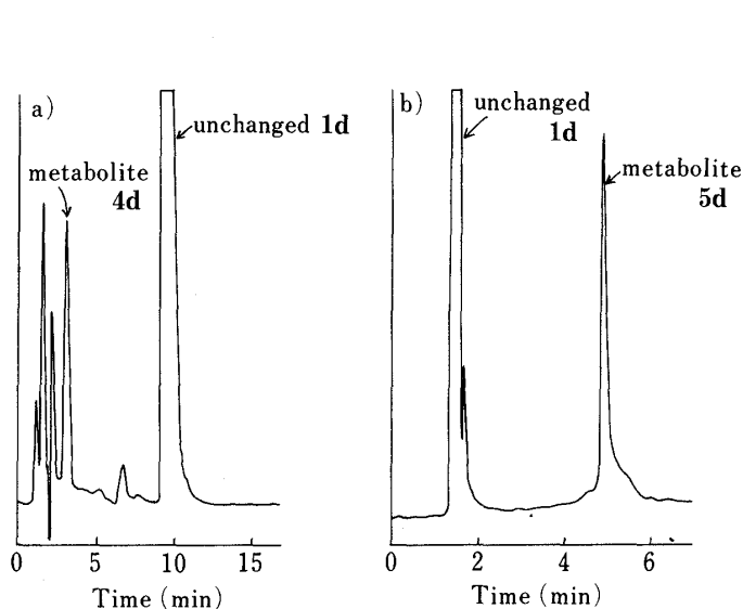
Fig. 5. HPLC of the Ethyl Acetate Extract of 5 H - N -Propyldibenz[ b,f ]azepine ( 1d ) Incubated with Rat Liver Microsomal Fractions
