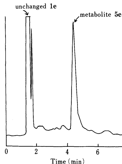
Fig. 6. HPLC of the Ethyl Acetate Extract of 5 H - N -Benzyldibenz[ b,f ]azepine ( 1e ) Incubated with Rat Liver Microsomal Fractions
