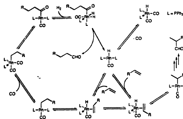
Scheme 1. Wilkinson's generally accepted mechanism of hydroformylation.
