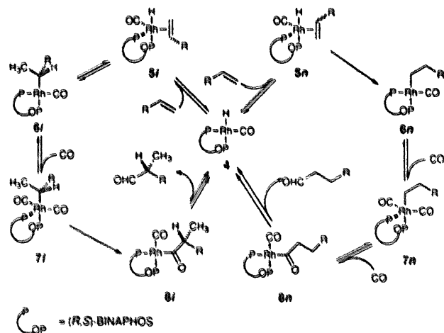
Scheme 2. A proposed mechanism for hydroformylation of 1f catalyzed by \text{Rh}(\text{I})\text{-(R,S)-BINAPHOS} .
