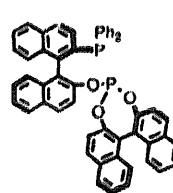
(R,S)-BINAPHOS
