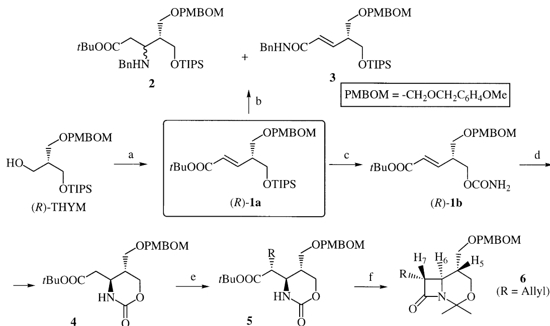
Scheme 1. (a) (i) (\text{COCl})_2 , DMSO, i\text{-Pr}_2\text{NH} , 92%; (ii) \text{Ph}_3\text{P}=\text{CHCO}_2\text{Bu}^t , 92% (two steps); (b) \text{Bn}(\text{TMS})\text{NLi} , THF, -78^{\circ}\text{C} ; (c) \text{Bu}_4\text{NF} , 80%; \text{ClSO}_2\text{NCO} , then \text{H}_2\text{O} , 85%; (d) t\text{-BuOK} (see text); (e) base, RX (see Table 1); (f) (i) \text{Boc}_2\text{O} , \text{Et}_3\text{N} , DMAP, \text{CH}_2\text{Cl}_2 , 94%; (ii) \text{Cs}_2\text{CO}_3 , MeOH, 88%; (iii) \text{KOH} , EtOH, 77%; (iv) \text{TIPS-Cl} , DBU, MeCN, 59%; (v) (\text{PyS})_2 , \text{PPh}_3 , MeCN, 90%; (vi) TBAF, THF, 44%; (vii) DME, \text{BF}_3 \cdot \text{Et}_2\text{O} , \text{CH}_2\text{Cl}_2 , 39%
