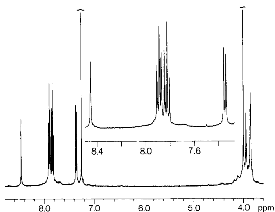
Fig. 2. 400-MHz ^1\text{H} -NMR spectrum of the NaBr cryptate of the macrobicyclic ligand 4b ([bpy( \text{CO}_2\text{Me} ) _2 ·bpy·bpy]) in \text{CDCl}_3 . Insert: expansion of the heterocyclic-moiety domain. Solvent at 7.25 ppm.
