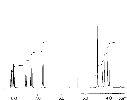
Fig. 1. 200-MHz ^1\text{H} -NMR spectrum of the LiBr cryptate of the macrobicyclic ligand 1 ([bpy·py·py]) in \text{CDCl}_3 . Solvent at 7.25 ppm; \text{CH}_2\text{Cl}_2 peak at 5.3 ppm.
