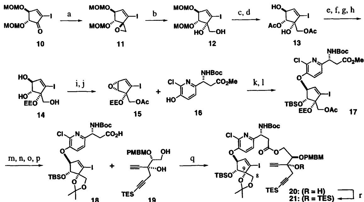
Scheme 2. Reagents and conditions: (a) \text{Me}_3\text{SiI} , n\text{-BuLi} , THF, -85^\circ\text{C} to rt, 60%; (b) 5% \text{HClO}_4 (aq), THF, 61%; (c) \text{Ac}_2\text{O} , \text{Et}_3\text{N} , DMAP, \text{CH}_2\text{Cl}_2 , 91%; (d) PPTS, 2-butanone, reflux, 74%; (e) TBSCl, imidazole, DMF, 96%; (f) ethyl vinyl ether, PPTS, \text{CH}_2\text{Cl}_2 , 97%; (g) TBAF, THF, -40^\circ\text{C} , 85%; (h) \text{K}_2\text{CO}_3 , MeOH, 98%; (i) DIAD, \text{PPh}_3 , toluene; (j) \text{Ac}_2\text{O} , pyridine, 62% (two steps); (k) CsF, DMF, 60^\circ\text{C} ; (l) TBSCl, imidazole, DMF, 50^\circ\text{C} , 72% (two steps); (m) \text{K}_2\text{CO}_3 , MeOH, 91%; (n) PPTS, MeOH, 93%; (o) 2-methoxypropene, PPTS, DMF, 90%; (p) 0.33M KOH (aq), THF, MeOH, 96%; (q) EDC·HCl, DMAP, \text{CH}_2\text{Cl}_2 , 75%; (r) TESCl, imidazole, DMF, >99%. PMBM: p -methoxybenzyloxymethyl
