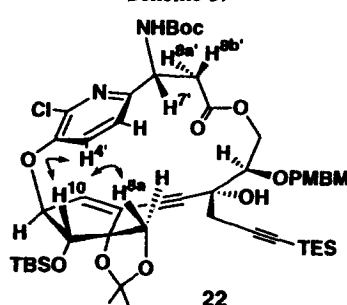
Figure 2. ROESY correlations of 22 (500 MHz, \text{CDCl}_3 )
