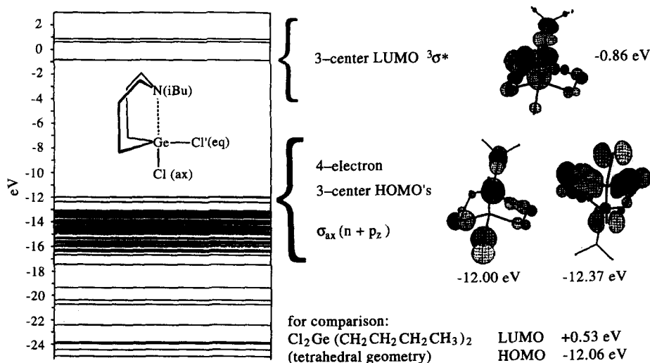
Fig. 3. Sequence of the MO's for the compound 4 in terms of CACAO-graphs [21a]. The LUMO and HOMO energies for the tetrahedral analogue Cl_2GeBu_2^2 are given for comparison [21b]. For the used nomenclature see ref. [6], for the extended Hückel parameters see ref. [22].
