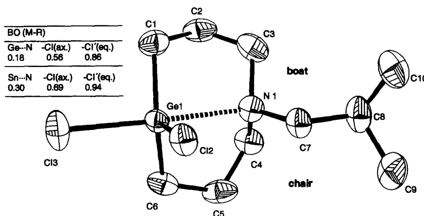
Fig. 1. Ortep plot of the compound 4 (NBu'/Cl 2 ); thermal ellipsoids are at the 50% probability level. Hydrogen atoms are omitted for better clarity. The plot of the compound 3 (NBu'/Cl 2 ) looks nearly the same. The Pauling bond orders BO [15] at Ge and Sn are compared: three-times long distances for the germanium compound, and three-times short distances for its tin analogue.
