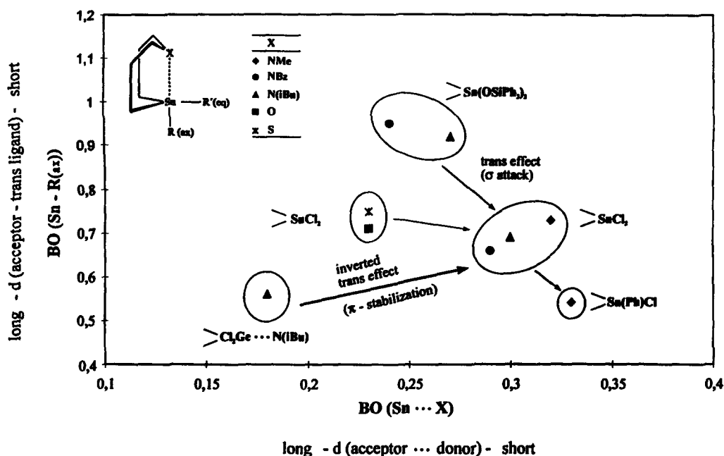
Fig. 2. Graph of the Pauling bond orders BO(Sn-R(ax)) vs BO(Sn \cdots X) for the compounds 3 and 4.
