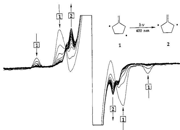
Figure 2. Photochemical isomerization of triplet 1 to triplet 2 by irradiation of 400 nm and 15 K. The matrix is methylcyclohexane.
