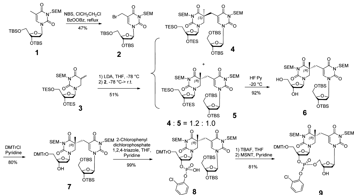
Scheme 1. Synthesis of the Protected R Isomer of SP TpT
