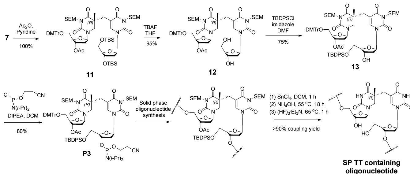
Scheme 4. Synthesis of the Dinucleoside SP TT-Containing Oligonucleotide via Phosphoramidite P3
