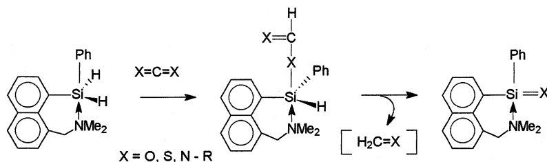
Scheme 4. Insertion and decomposition of heterocumulenes.
