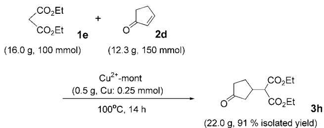
Scheme 2. Cu^{2+} -mont-catalyzed 100 mmol-scale Michael reaction under solvent-free conditions.
