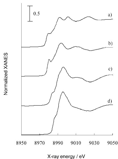
Figure 1. Normalized Cu K-edge XANES spectra of (a) Cu foil, (b) \text{Cu}_2\text{O} , (c) \text{CuO} , and (d) \text{Cu}^{2+} -mont.
