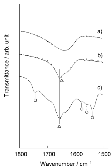
Figure 4. IR spectra of a) fresh Cu 2+ -mont, b) the Cu 2+ -mont after treatment with 2a , and c) the Cu 2+ -mont after treatment with both 2a and 1c . Δ: coordinated 2a (1658 cm -1 ); ○: acetylacetonato-Cu species (1580, 1558, and 1539 cm -1 , ref. [43]); □: free 1c (1747 cm -1 ). The fresh Cu 2+ -mont (0.2 g) was treated with 2a (1.0 equiv Cu) in nitromethane (1 mL). The 2a -covered Cu 2+ -mont was further reacted with one equivalent of 1c .
