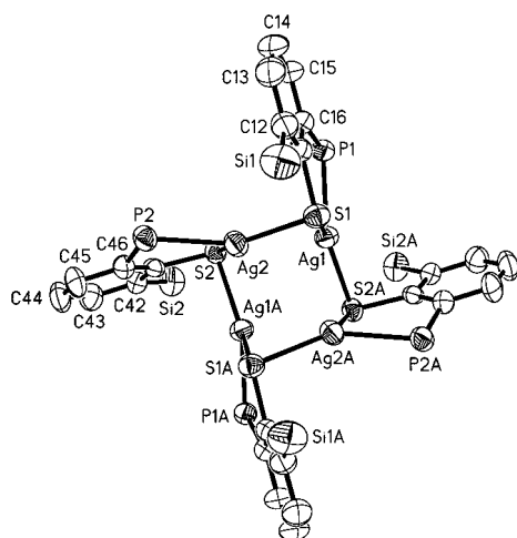
Figure 3. Perspective view of the coordination spheres of the metals in [\text{Ag}_4\{2\text{-(Ph}_2\text{P)}\text{-6-(Me}_3\text{Si)C}_6\text{H}_3\text{S}\}_4] ( 5 ).
