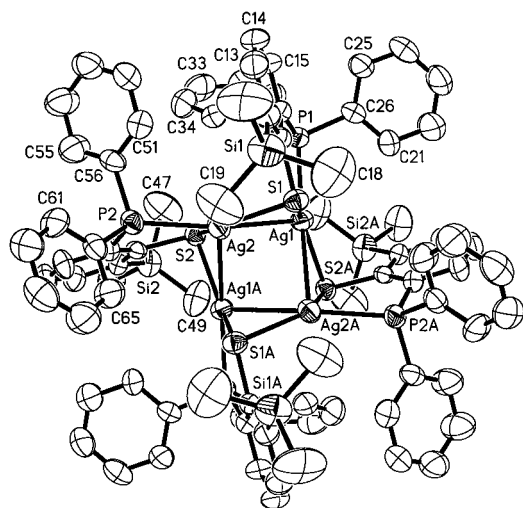
Figure 2. An ORTEP view of the structure of [\text{Ag}_4\{2\text{-(Ph}_2\text{P)}\text{-6-(Me}_3\text{Si)C}_6\text{H}_3\text{S}\}_4] ( 5 ).
