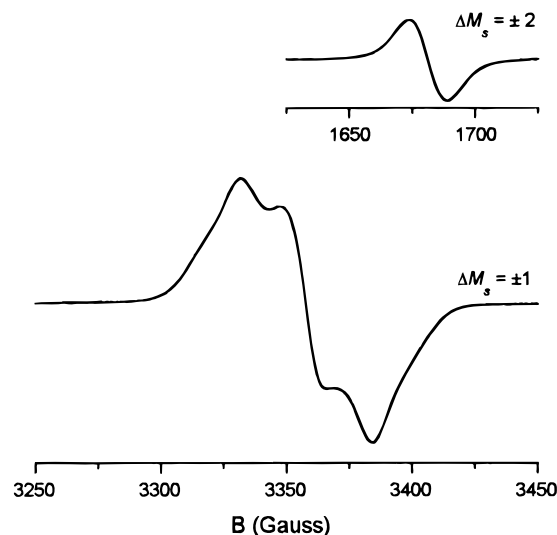
Figure 2. X-Band ESR spectrum of 1^{2+2+} in \text{CH}_2\text{Cl}_2/\text{TFA} recorded at 110 K. The central line is due to some doublet impurity. Inset: \Delta M_s = \pm 2 transition recorded at 4.0 K.
