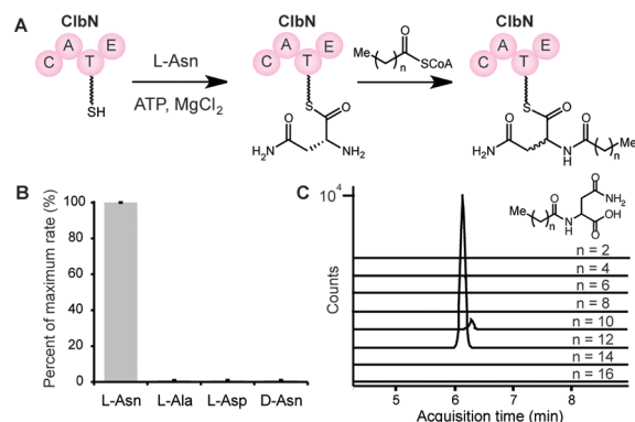
Figure 2. ClbN is an NRPS involved in constructing the prodrug scaffold. (A) Biosynthetic hypothesis for the activity of ClbN. (B) ATP–[ 32 P]PP i exchange assay for ClbN substrate specificity. (C) Extracted ion chromatograms of products obtained from the LC–MS competition assay with ClbN, L-Asn, and equal amounts of C 4 –C 18 fatty acyl-CoA substrates. All traces have been scaled to the same intensity.
